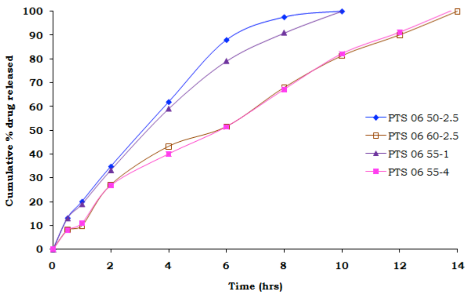
Figure 6 Dissolution profile of TSFT of PTS 06.
