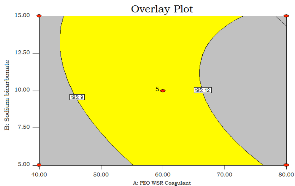
Figure 19 Overlay plot for the optimization of thermally sintered floating tablets of propranolol HCl.
